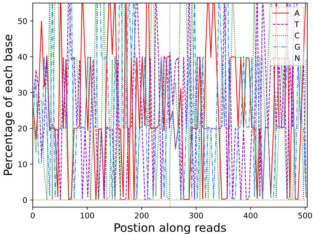
Base percentage along reads (R10429)
